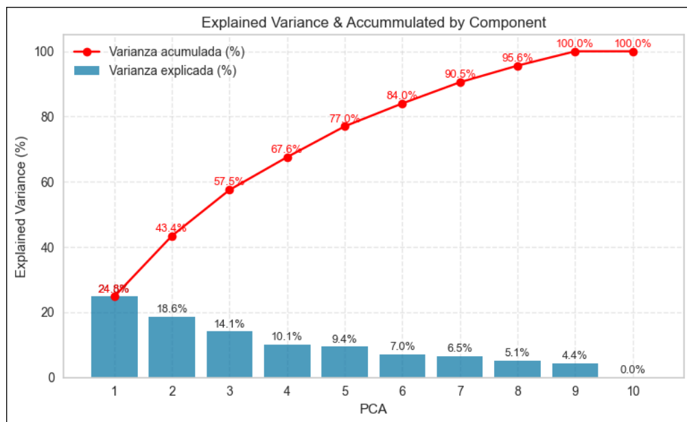
Figure 3.28: Cumulative Explained Variance (PCA) . Source: Author’s own elaboration.
