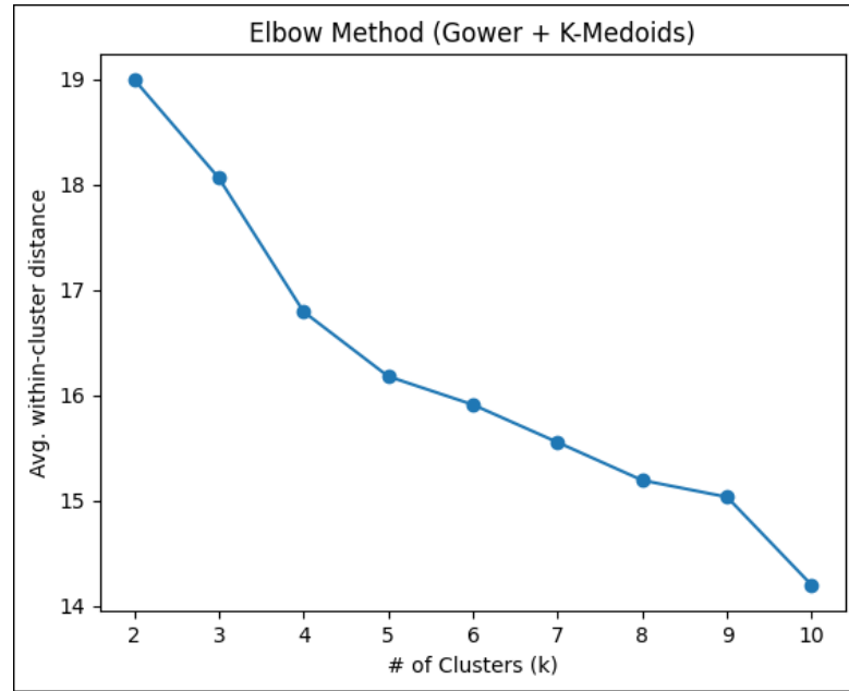
Figure 3.25: Elbow plot. Source: Author's own elaboration.
