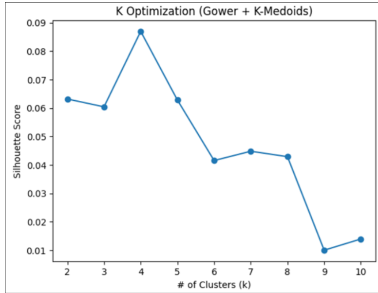
Figure 3.26: Silhouette scores and plot. Source: Author's own elaboration.
