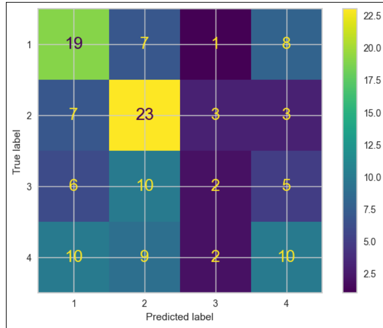
Figure 3.31: Confusion matrix of final model. Source: Author's own elaboration.
